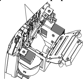
Using cross screwdriver to adjust the two screws for the adjustment the lamp's position
