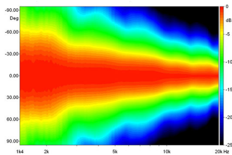
VERTICAL BEAMWIDTH
