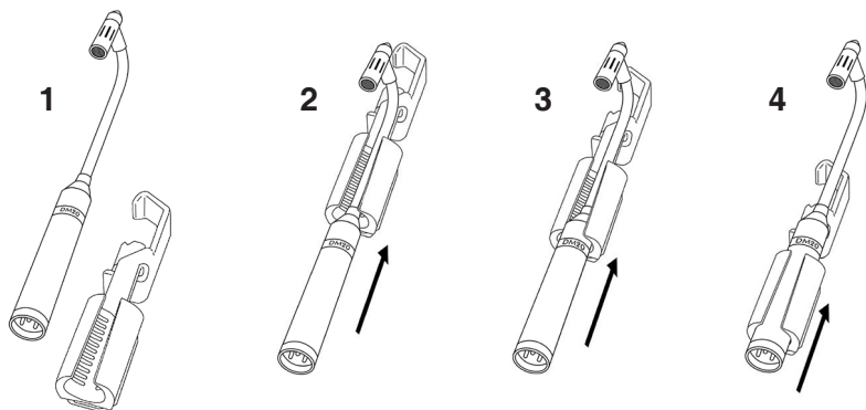
Figure 5 Inserting the DM20 DrumMic™ into the RimMount™
