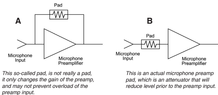
Figure 1-A and 1-B Types of Preamp Input Pads
