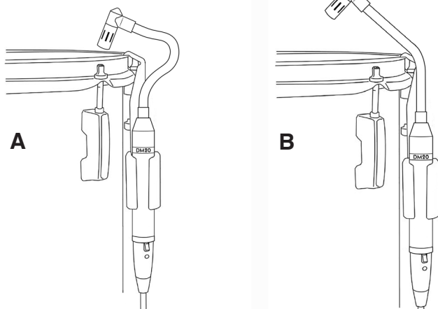
Figure 10-A and 10-B Miking the Top Head of a Tom
