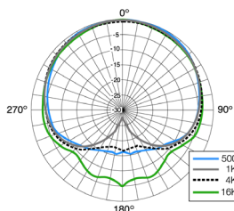
DM20 Polar Response
